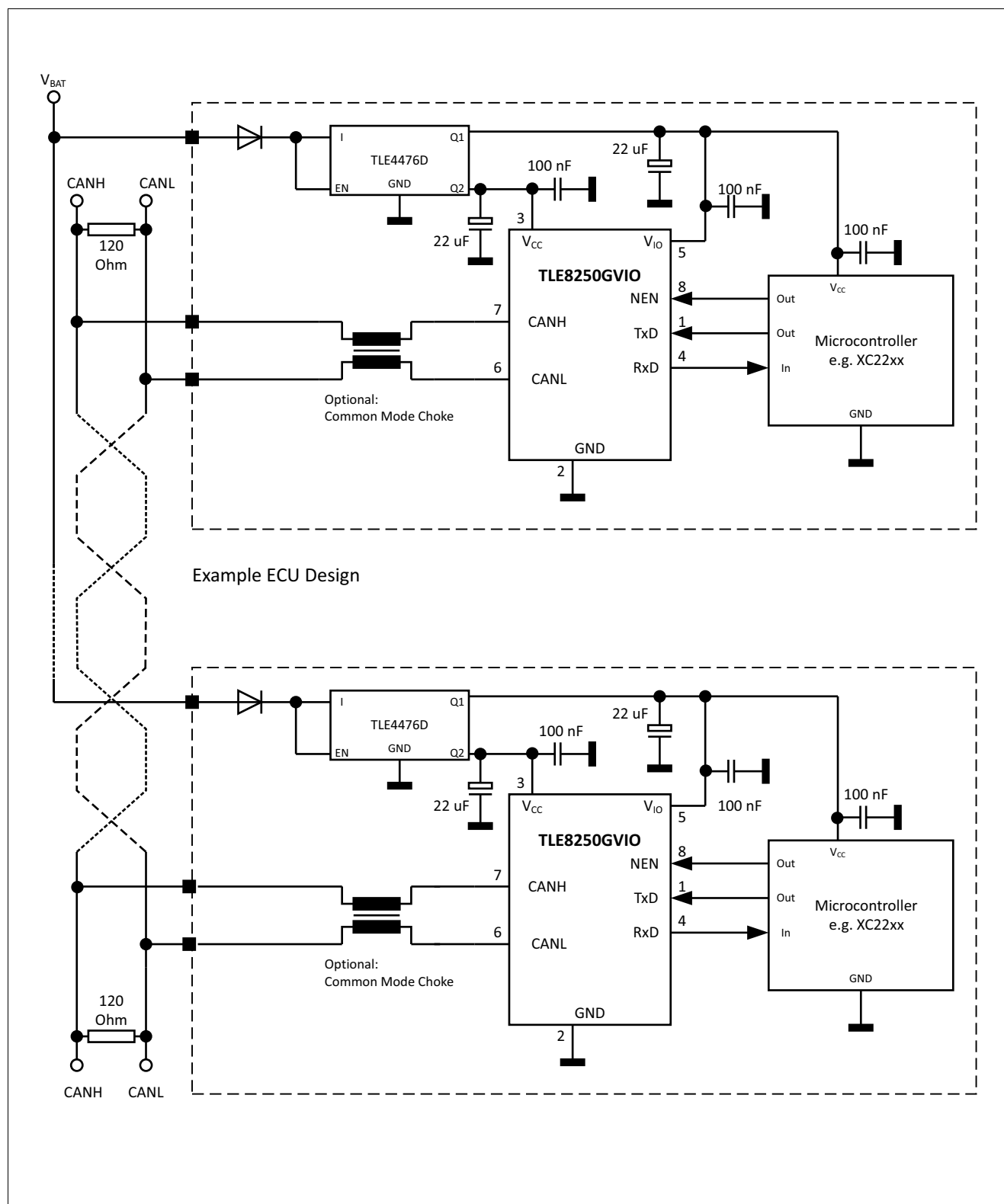
Figure 10 Simplified Application for the TLE8250GVIO
