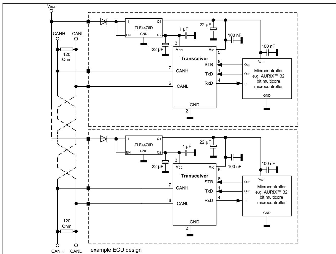
Figure 14 Application circuit
