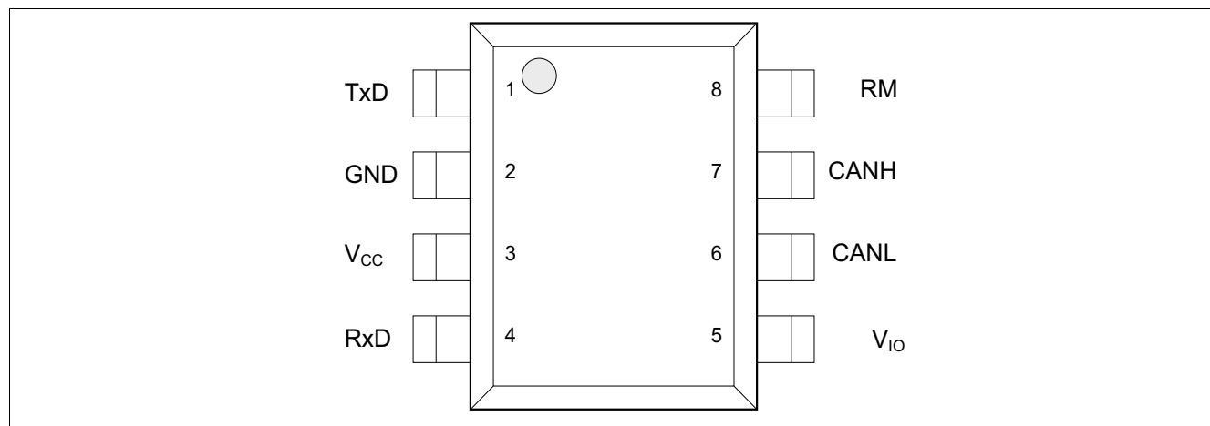
Figure 2 Pin assignment
