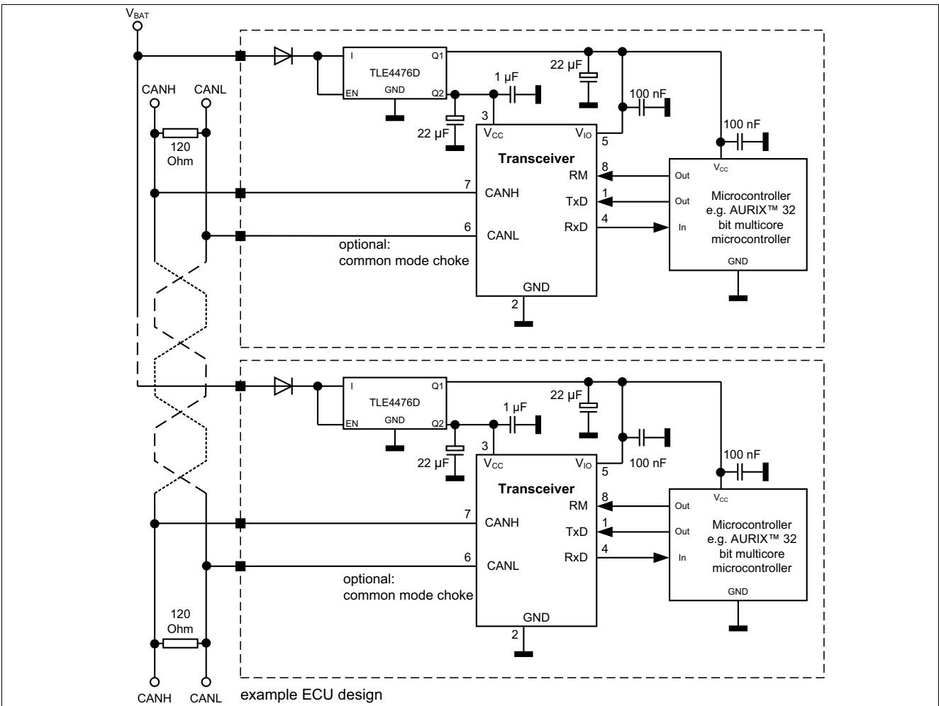
Figure 12 Application circuit
