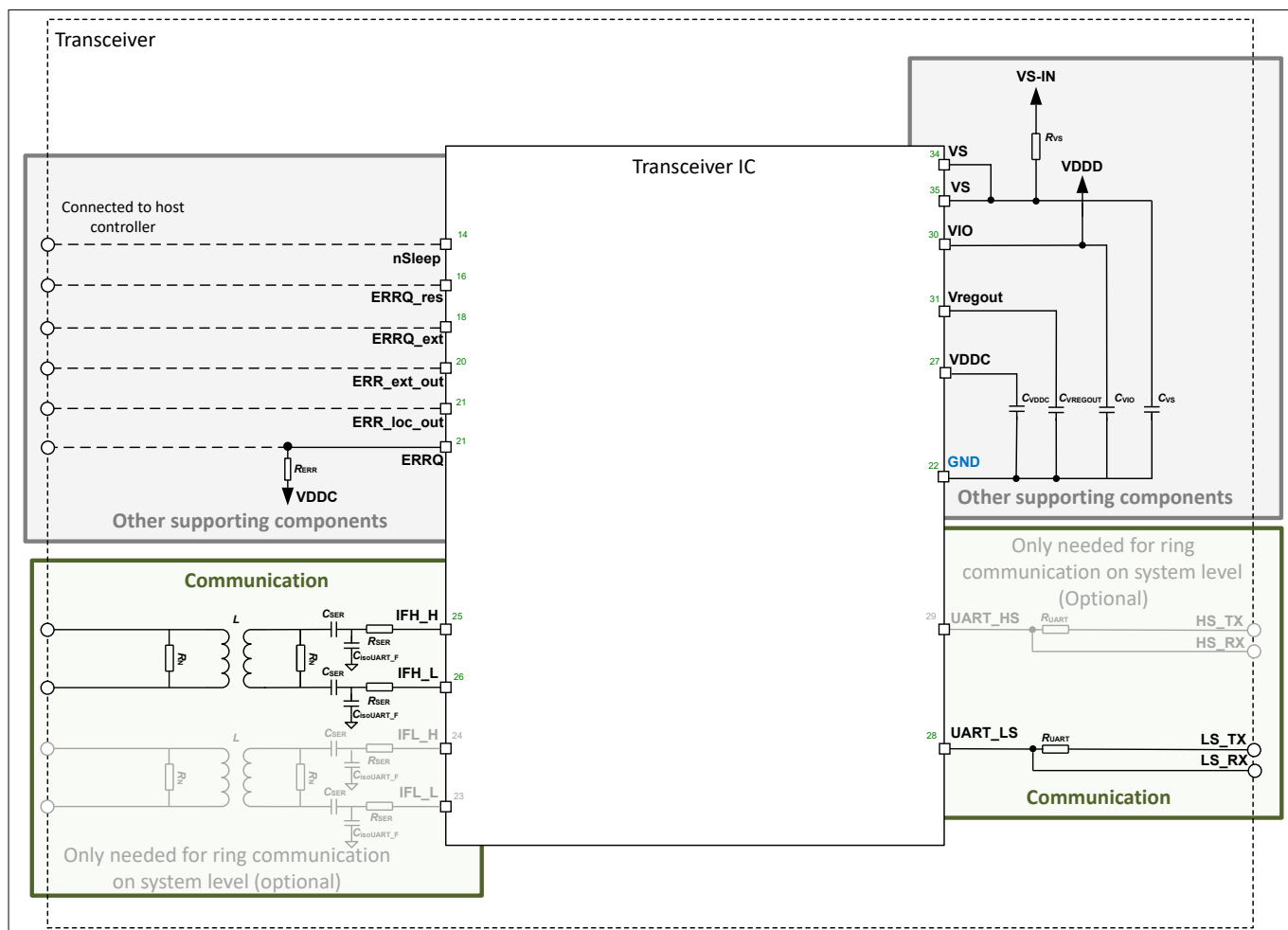
Figure 7 External circuitry transceiver IC
