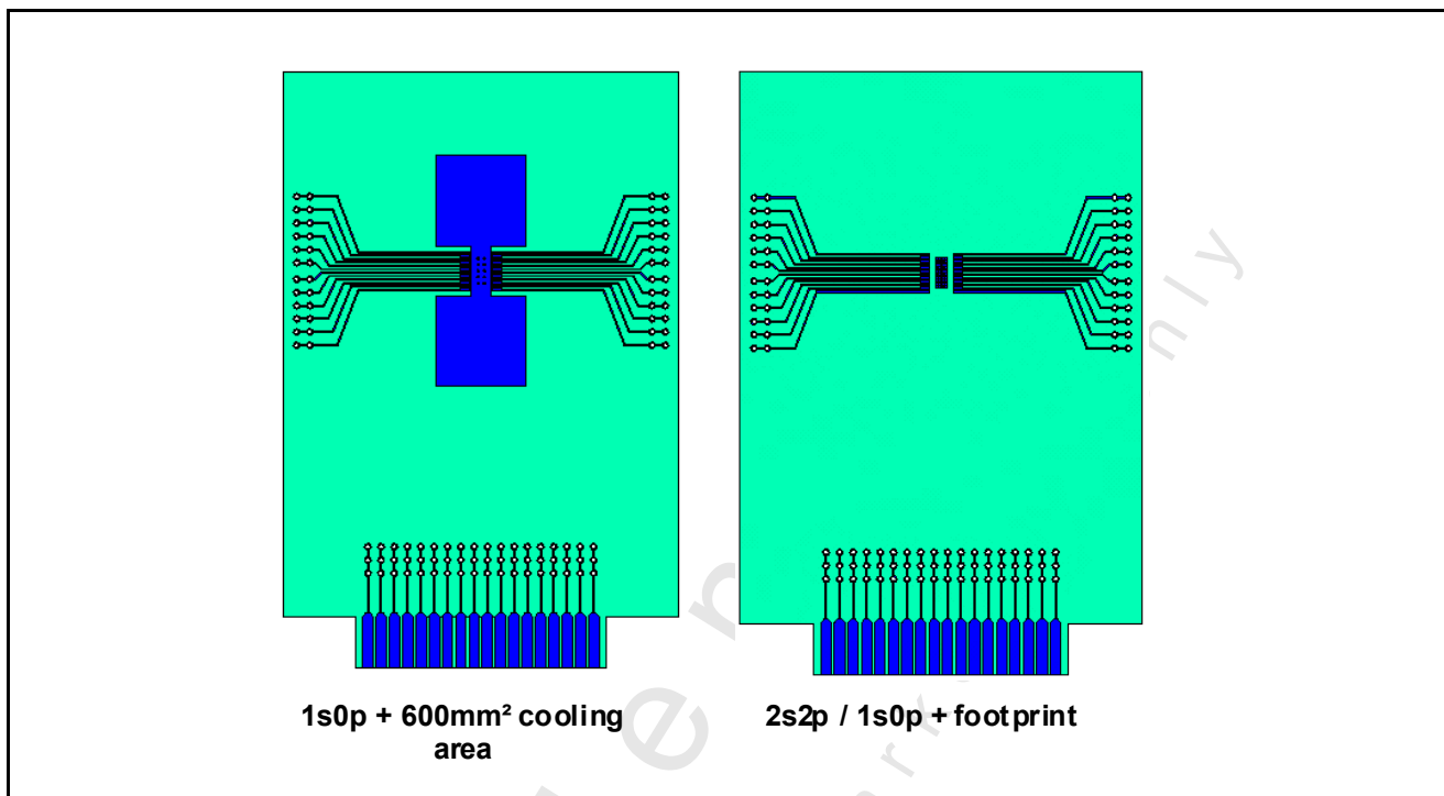
Figure 20 Board Setup
