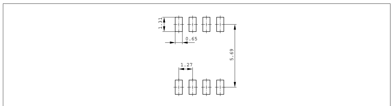
Figure 13 Footprint
