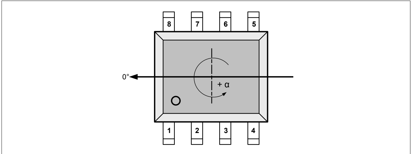
Figure 3 Pin-out of the discrete TMR bridge
