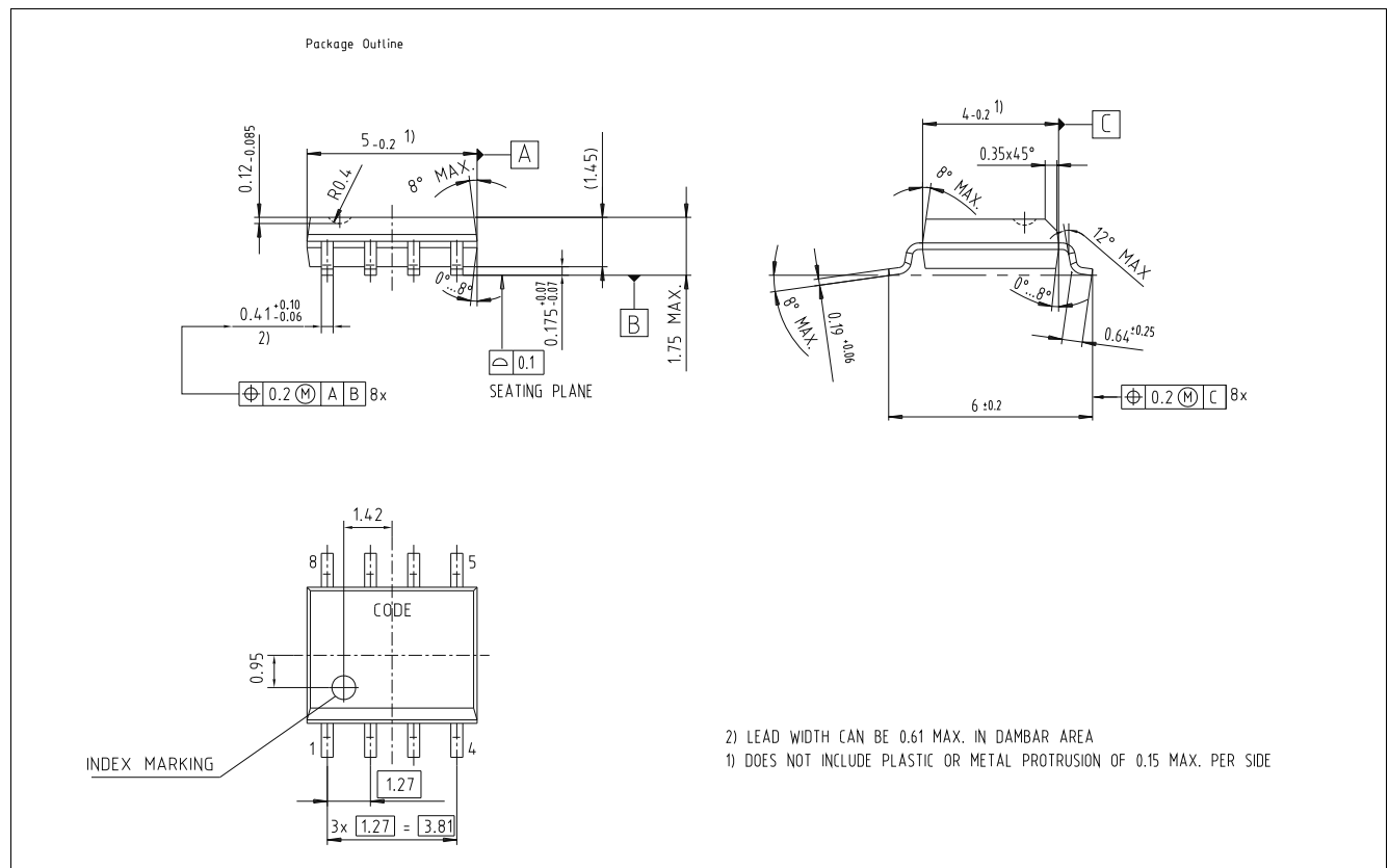
Figure 12 Package outline
