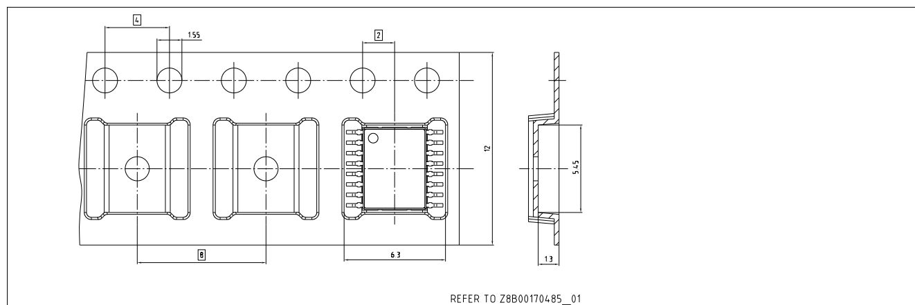
Figure 7 Tape and Reel
