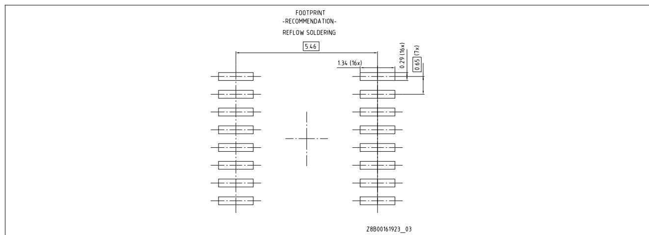
Figure 6 Footprint of PG-TDSO-16
