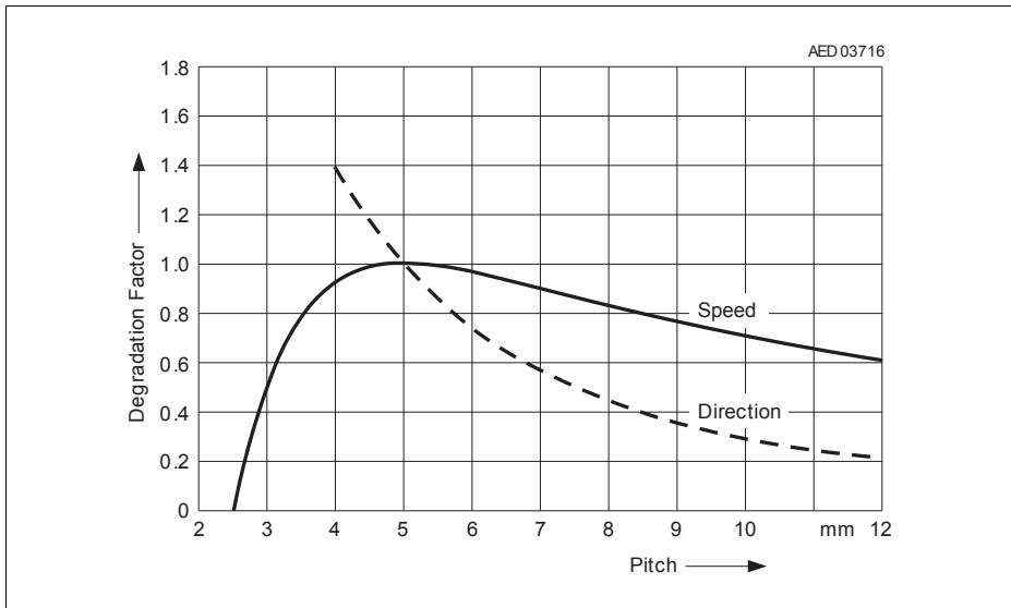
Figure 15 Degradation of speed and direction signal at sinusoidal input signals = f_{(\text{pitch})}
