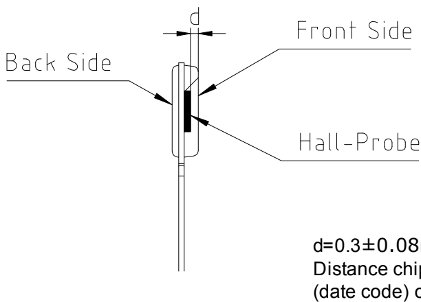
Figure 12 Distance Chip to Upper Side of IC
