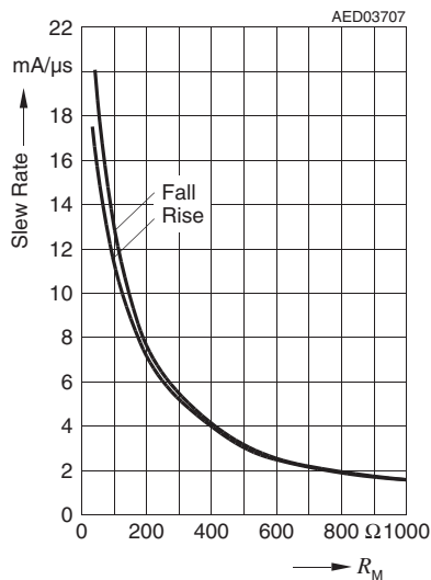
Slew Rate with C = 1.8 \text{ nF} = f(R_M)
