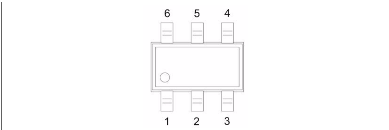
Figure 2 TLE493D-W2B6 pinout
