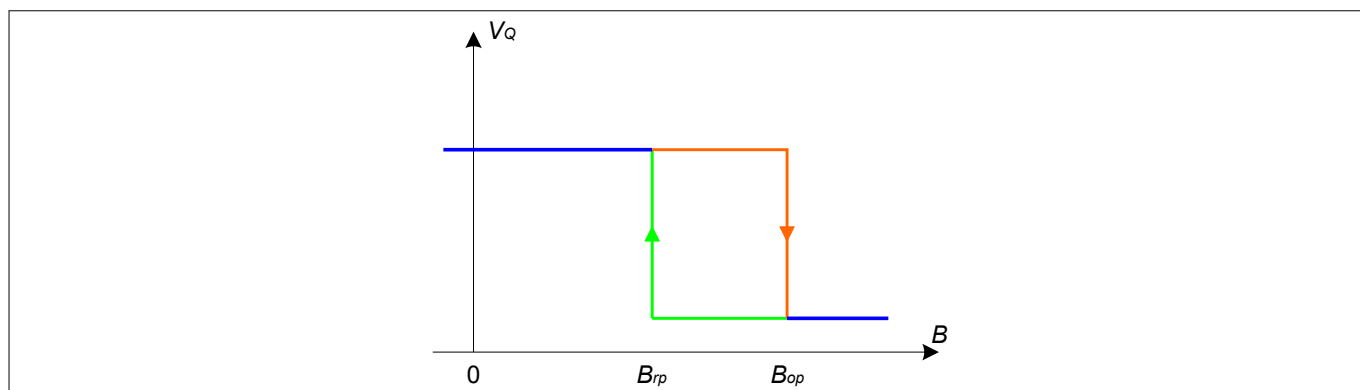
Figure 4 Output signal
