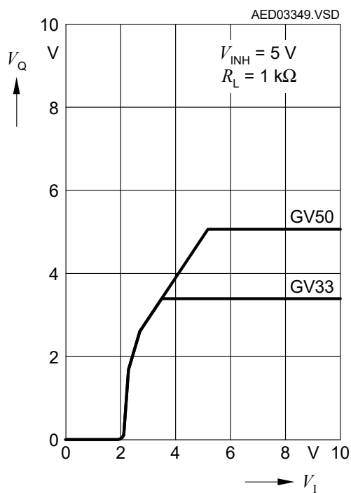
Output voltage V_Q vs. input voltage V_I
