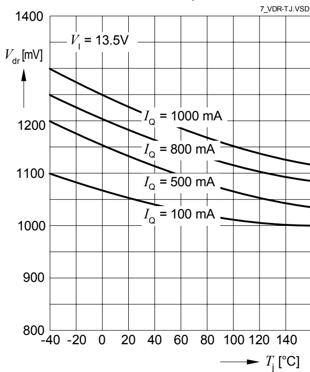
Dropout Voltage V_{\text{DR}} versus Junction Temperature T_j
