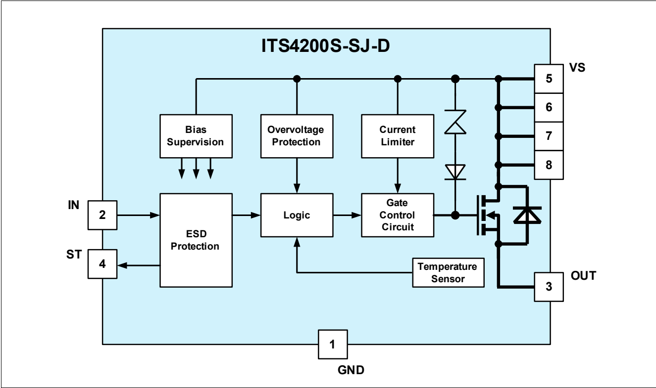
Figure 1 Block diagram
