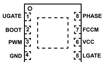
ISL95808 (8 LD 2x2 DFN) TOP VIEW
