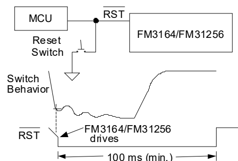
Figure 4. Manual Reset
