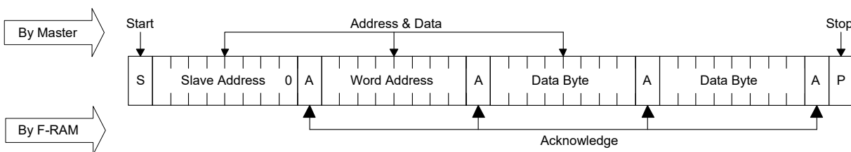
Figure 8. Multi-Byte Write
