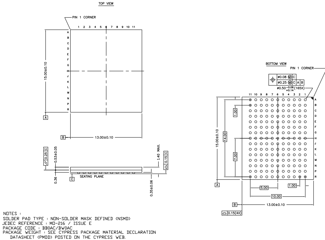
图 6. 165 脚 FBGA (13 × 15 × 1.4 mm) BB165D/BW165D (0.5 脚直径) 封装外形, 51-85180
