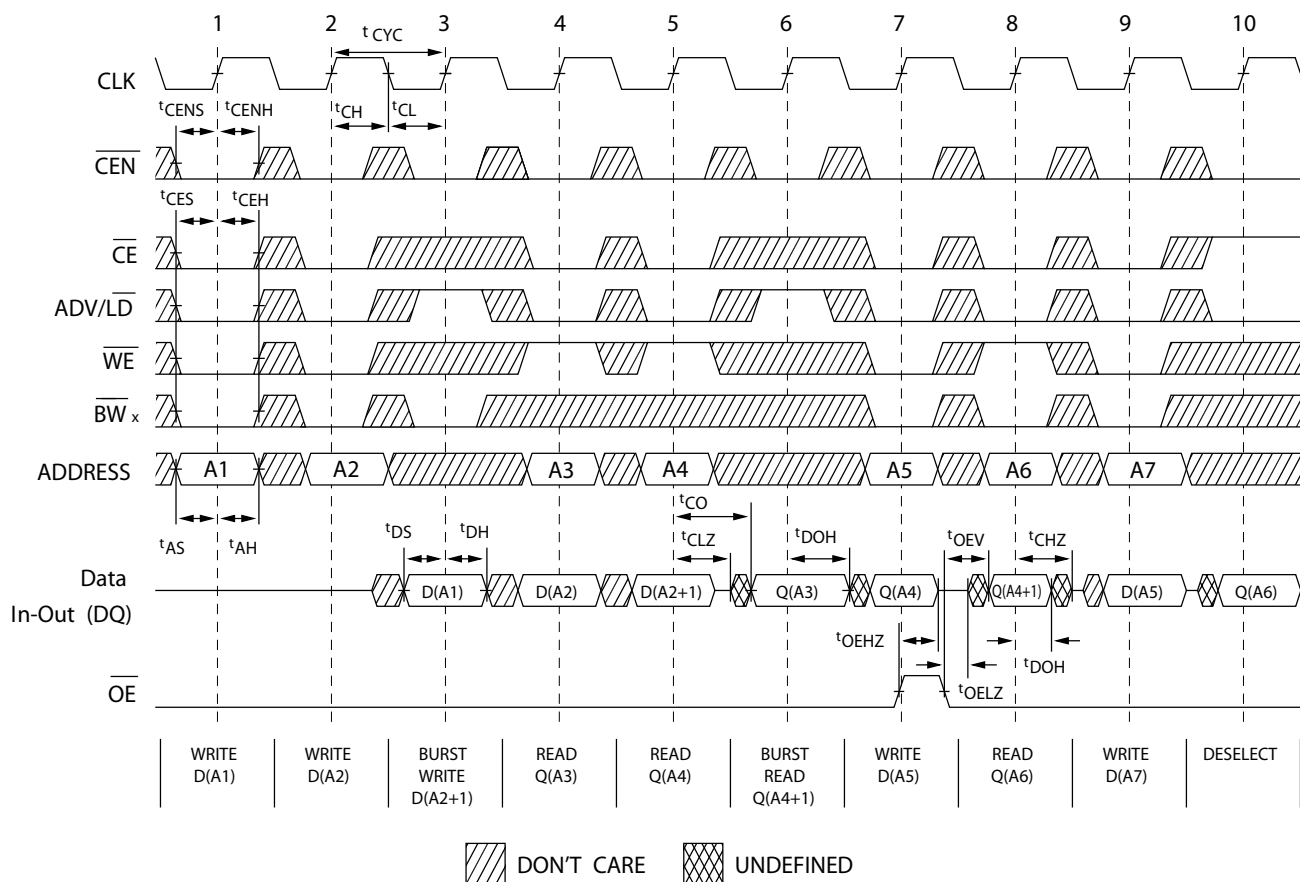
Figure 4. Read/Write/Timing [26, 27, 28]
