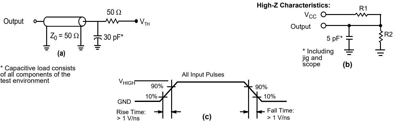
Figure 7. AC Test Loads and Waveforms [14]
