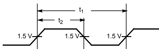
Figure 2. All Outputs Rise/Fall Time
