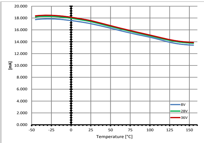
Sense Signal Maximum Current in Fault
