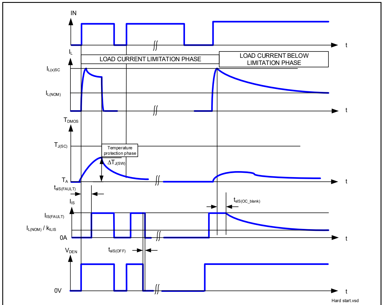
Figure 18 Overload Protection
