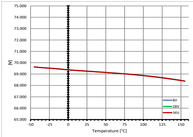
Sense Signal Maximum Voltage
