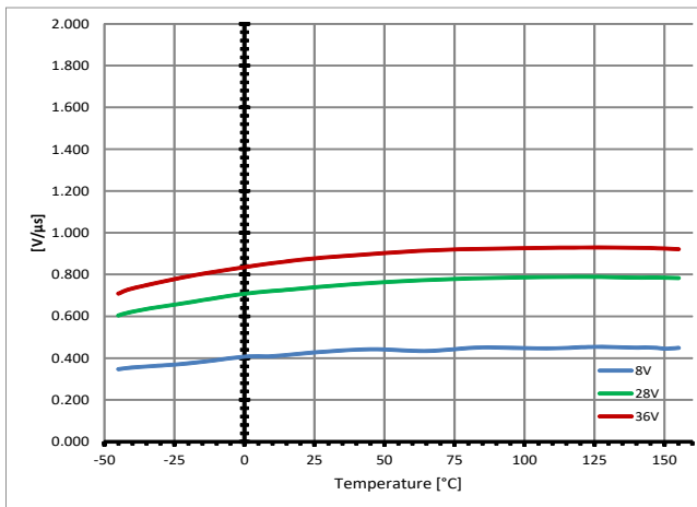
Slew Rate at Turn ON dV/dt_{ON} = f(T_J; V_S), R_L = 25 \Omega
