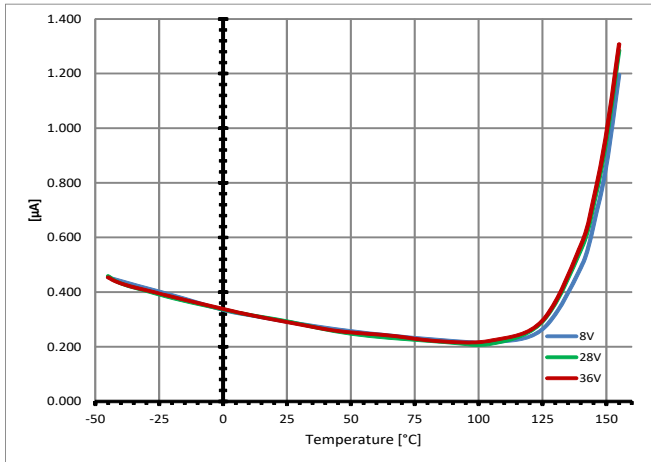
Current Sense at no Load
