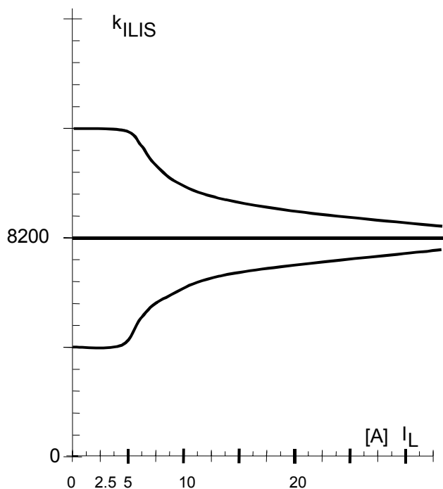
Figure 6b: Current sense ratio 12) :
