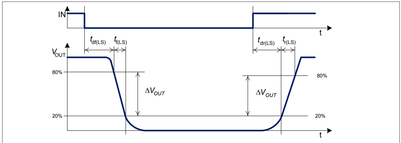
Figure 9 Definition of switching times low-side ( R_{load} to V_S )
