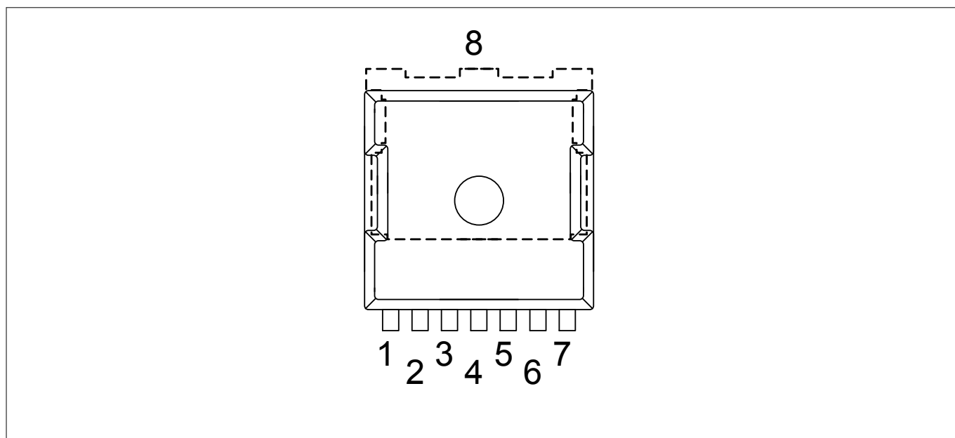
Figure 4 Pin assignment BTN9990LV (top view)
