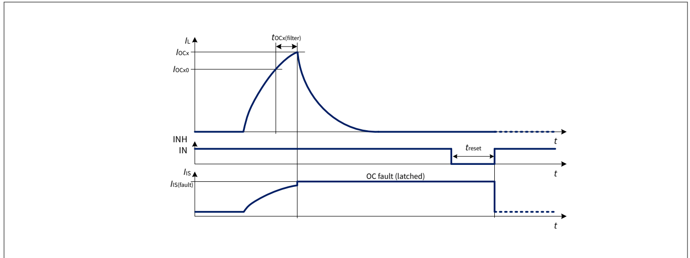
Figure 12 Timing diagram switch-OFF with latch (inductive load)
