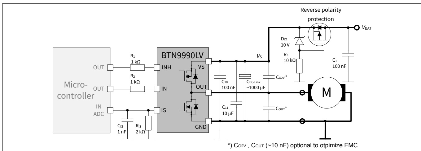
Figure 1 Typical application
