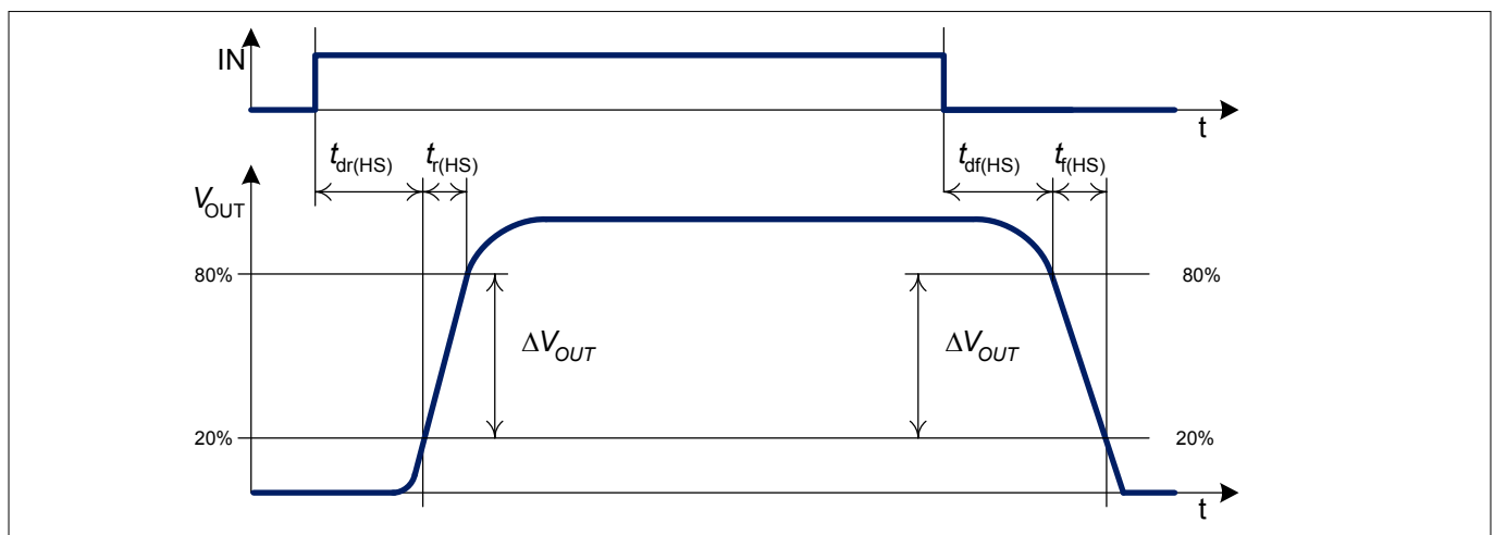
Figure 8 Definition of switching times high-side ( R_{\text{load}} to GND)
