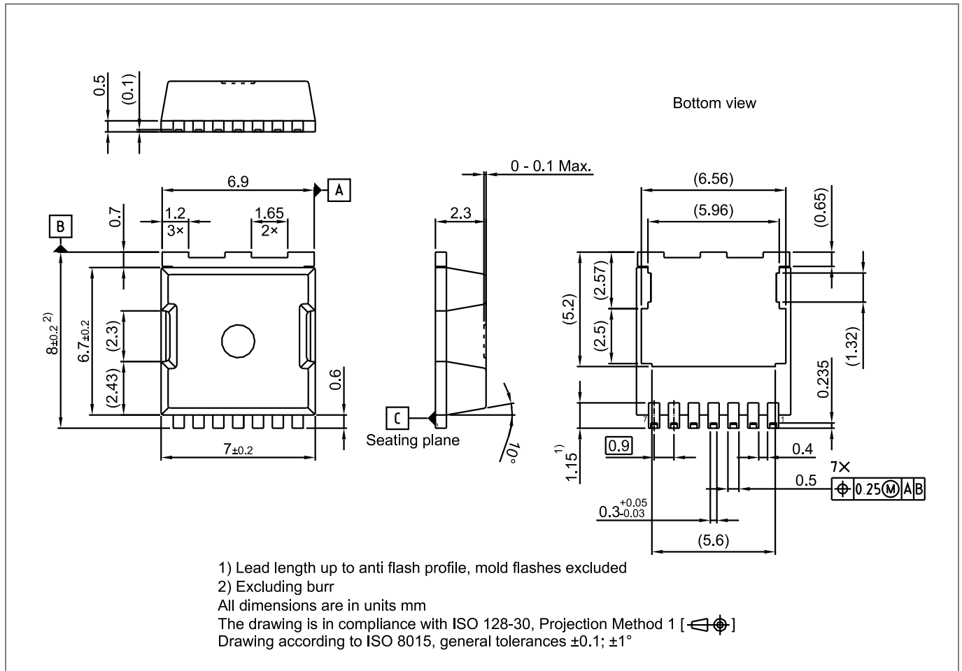
Figure 19 PG-HSOF-7 (sTOLL)
