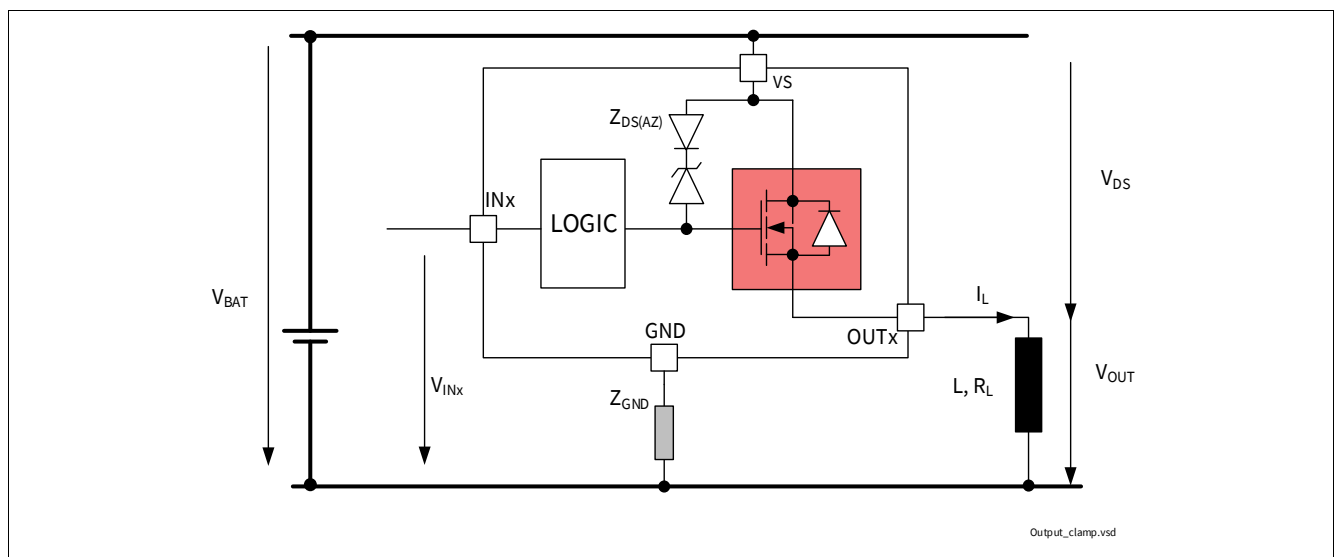
Figure 11 Output Clamp
