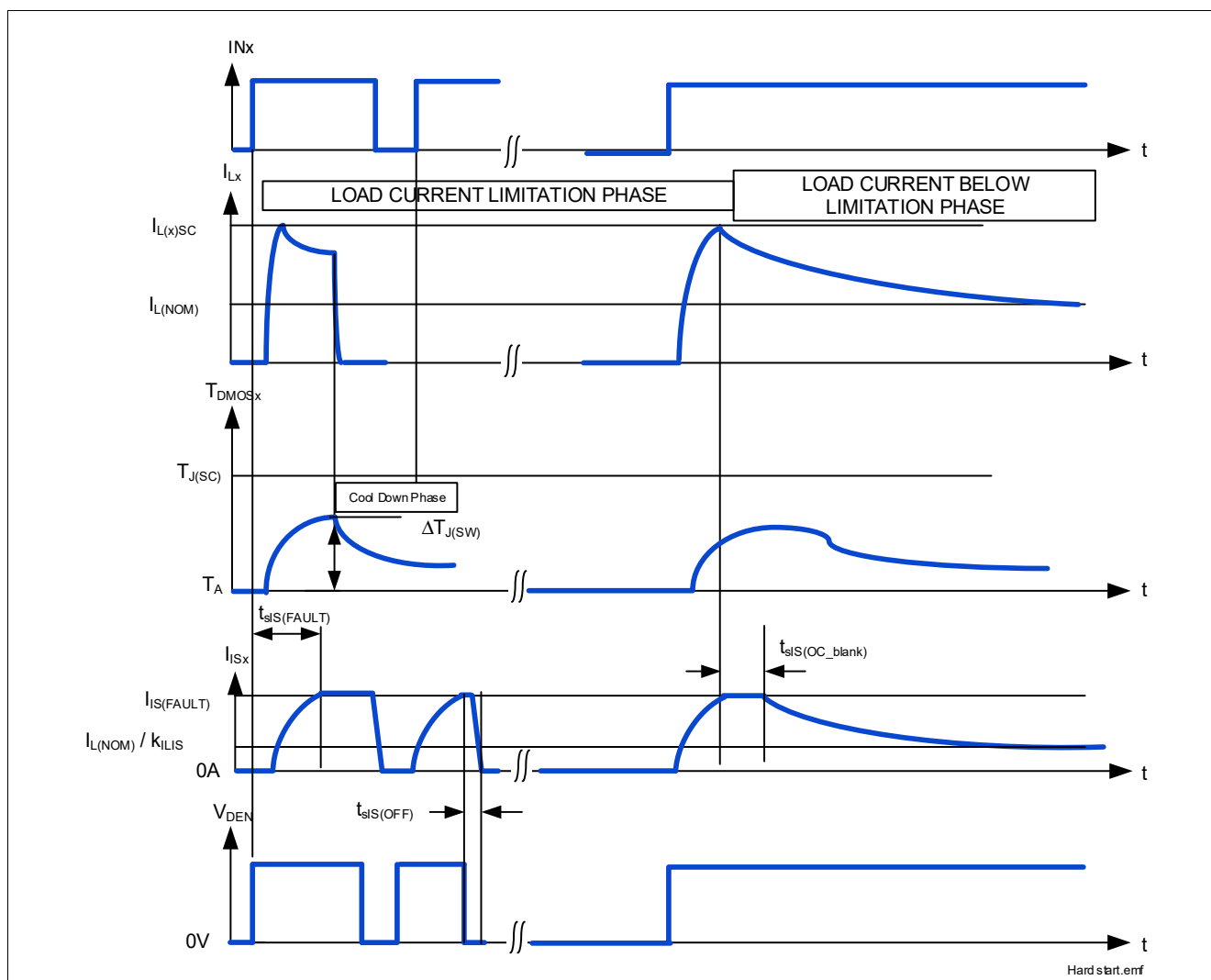
Figure 19 Overload Protection
