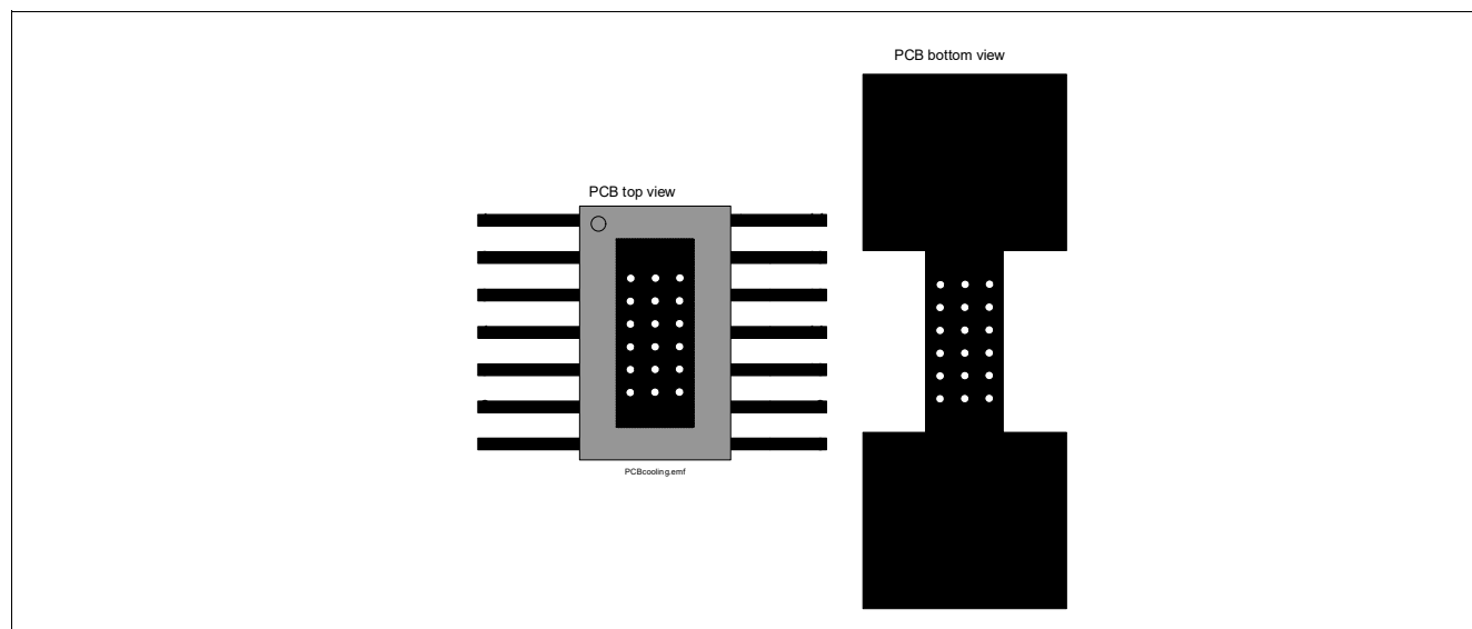
Figure 6 PC Board Top and Bottom View for Thermal Simulation with 600 mm² Cooling Area
