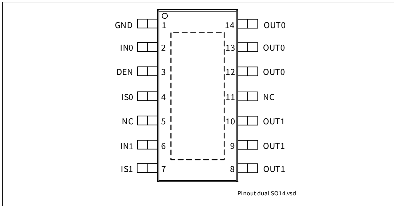
Figure 2 Pin Configuration
