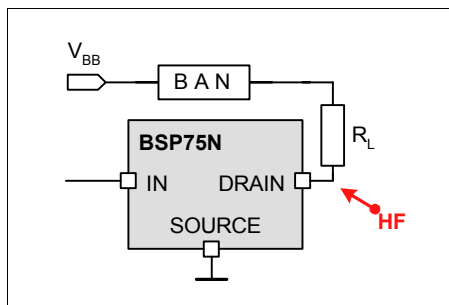
Test circuit for conducted susceptibility 2)
